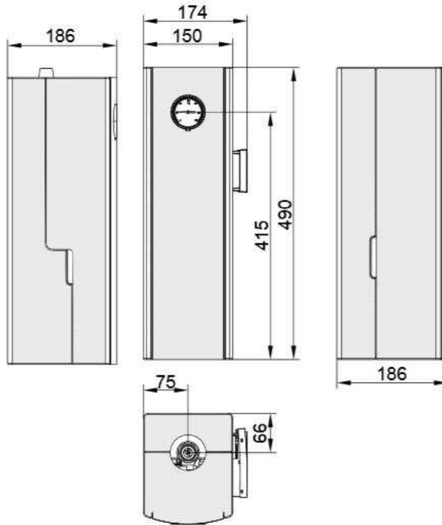
Solar-Pumpenstrang
